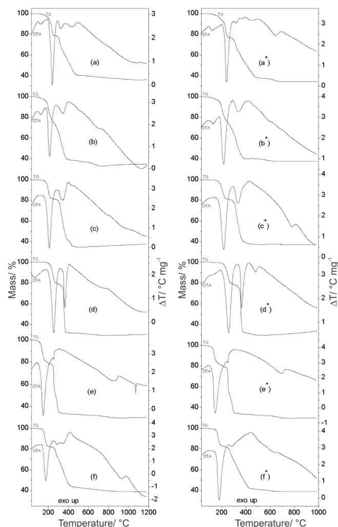
Figure 3. TG-DTA curves of the compounds in dynamic N_2 and CO_2^* atmospheres: (a, a*) MnL \cdot 2.5H_2O ( m = 7.126 mg; 7.024 mg *), (b, b*) FeL \cdot 2.5H_2O ( m = 7.145 mg; 7.009 mg*), (c, c*) CoL \cdot 2H_2O ( m = 7.089 mg; 7.242 mg*), (d, d*) NiL \cdot 2H_2O ( m = 7.148 mg; 7.182 mg*), (e, e*) CuL \cdot 2H_2O ( m = 7.079 mg; 7.329 mg*) and (f, f*) ZnL \cdot 2H_2O ( m = 7.295 mg; 7.085 mg*).
