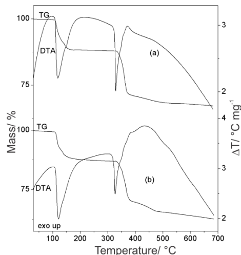
Figure 2. Simultaneous TG-DTA curves of the sodium malonate in (a) N_2 (7.069 mg) and (b) CO_2 (7.084 mg), atmospheres.
