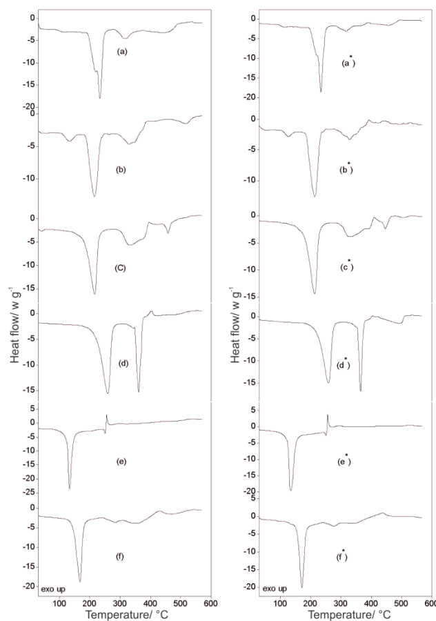
Figure 4. DSC curves of the compounds in dynamic N 2 and CO 2 * atmospheres: (a, a*) MnL·2.5H 2 O (m = 2.041 mg; 2.082 mg*), (b, b*) FeL·2.5H 2 O (m = 2.049 mg; 2.088mg*), (c, c*) CoL·2H 2 O (m = 2.035 mg, 2.093 mg*), (d, d*) NiL·2H 2 O ( m = 2.060 mg, 2.028 mg*), (e, e*) CuL·2H 2 O (m = 2.057 mg; 2.147 mg* ) and (f, f*) ZnL·2H 2 O (m = 2.050 mg, 2.180 mg*).
