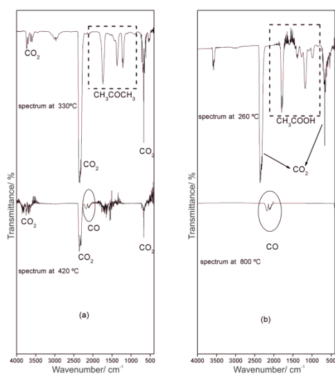
Figure 5. IR spectra of gaseous products evolved during the decomposition of the compounds: (a) CoL·2H 2 O, (b) CuL·2H 2 O.
