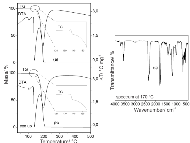
Figure 1. Simultaneous TG-DTA curves in dynamic (a) N_2 ( m = 7.116 mg), (b) CO_2 (7.132) atmospheres and (c) IR spectrum of the gases released during the decomposition of malonic acid in N_2 atmospheres.
